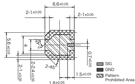
PCB Land Reference Dimensions
