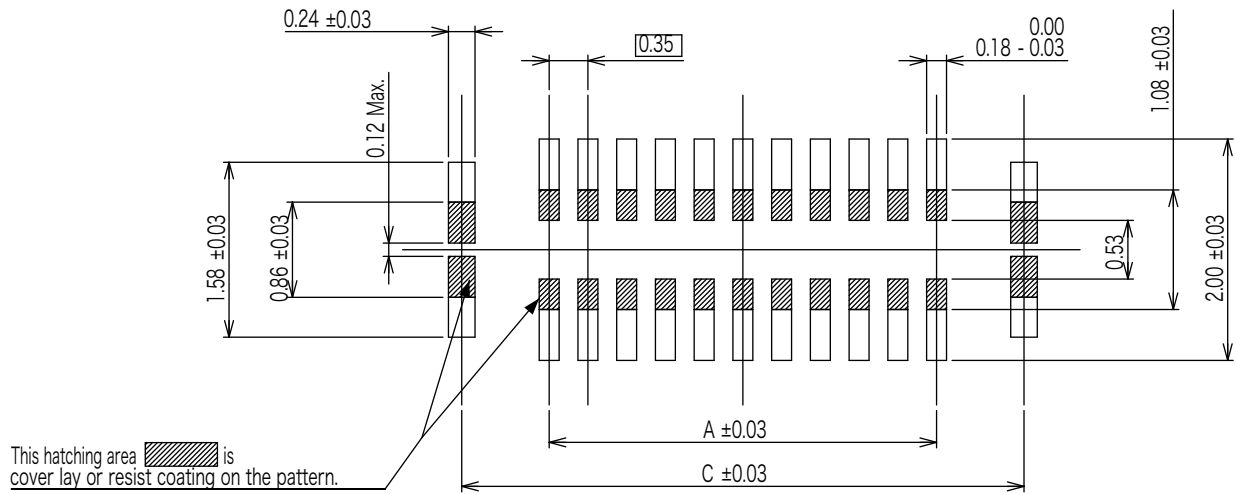
Reference P.C.B Layout (Connector Mounting Side View)
