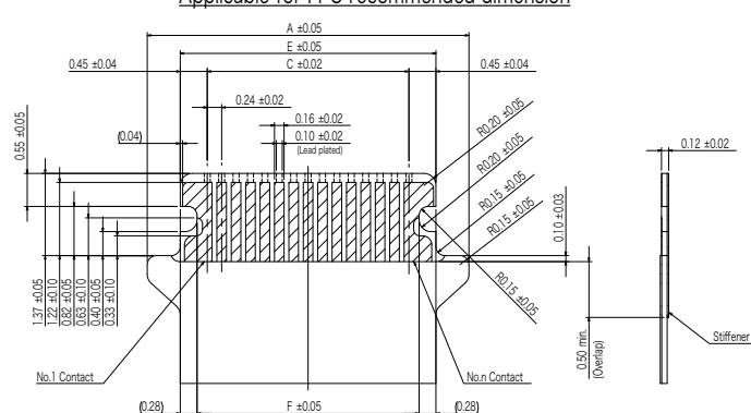
Applicable for FPC recommended dimension
