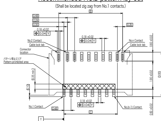
Part Number Number of Contact A B C D E F FF53-12A-R11A-B-3J 12 4.64 3.34 2.64 3.59 3.54 2.98
